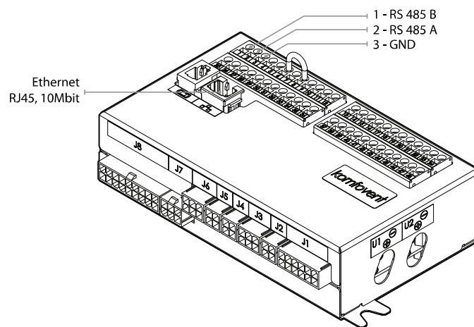
Picture 1. C5 controller board
